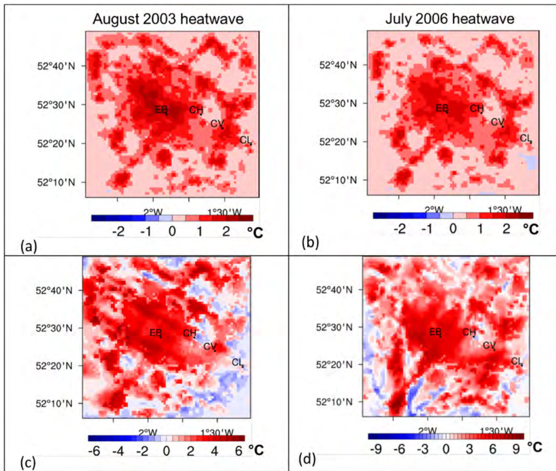
Fig. 4. Mean UHI intensity for the whole time-period across the West Midlands (a) 2nd–10th August 2003, and (b) 16th–27th July 2006. Snapshots of high UHI intensity for each period are shown in (c) 11 pm 5th August 2003, and (d) 11 pm 17th July 2006. Lettered points show monitoring stations used for model validation. EB = Edgbaston; CH = Coleshill; CV = Coventry; CL = Church Lawford. Note that the colour scales are not all equal. (For interpretation of the references to colour in this figure legend, the reader is referred to the web version of this article.)
