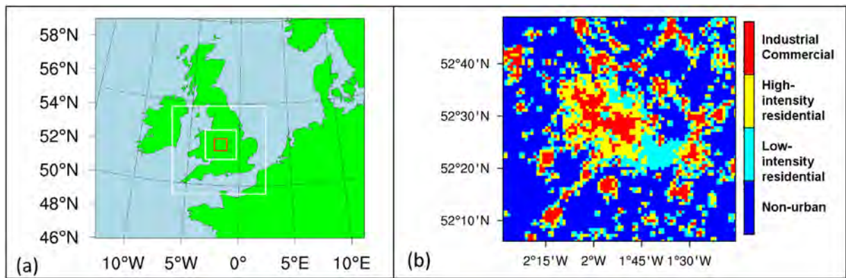
Fig. 1. (a) The domains covered by the WRF model simulation. The central domain (red box) is expanded in Fig. 1(b); (b) Urban classifications used in the urban canopy scheme in the WRF model in the central domain. The area shown covers approximately 80 \times 80 km. (For interpretation of the references to colour in this figure legend, the reader is referred to the web version of this article.)
