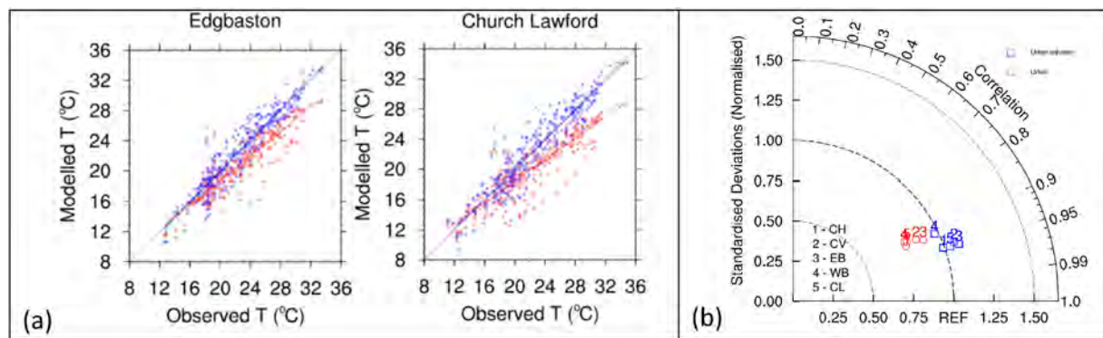
Fig. 2. (a) Modelled and observed ambient temperatures at MIDAS sites across the West Midlands in July 2006. (b) Taylor diagram showing statistical comparison between adjusted and unadjusted model. Unadjusted simulation is shown in red, and simulation with reduced initial moisture is shown in blue. A better comparison with observations is indicated by proximity to 'REF' on the horizontal axis. (For interpretation of the references to colour in this figure legend, the reader is referred to the web version of this article.)
