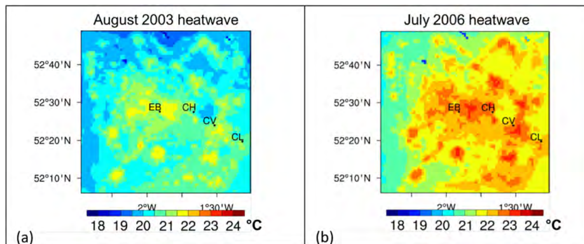
Fig. 3. Mean 2 m air temperatures simulated across the West Midlands during (a) heatwave period from 2nd–10th August 2003, and (b) for the heatwave period during 16th–27th July 2006. Lettered points show monitoring stations used for model validation. EB = Edgbaston; CH = Coleshill; CV = Coventry; CL = Church Lawford.
