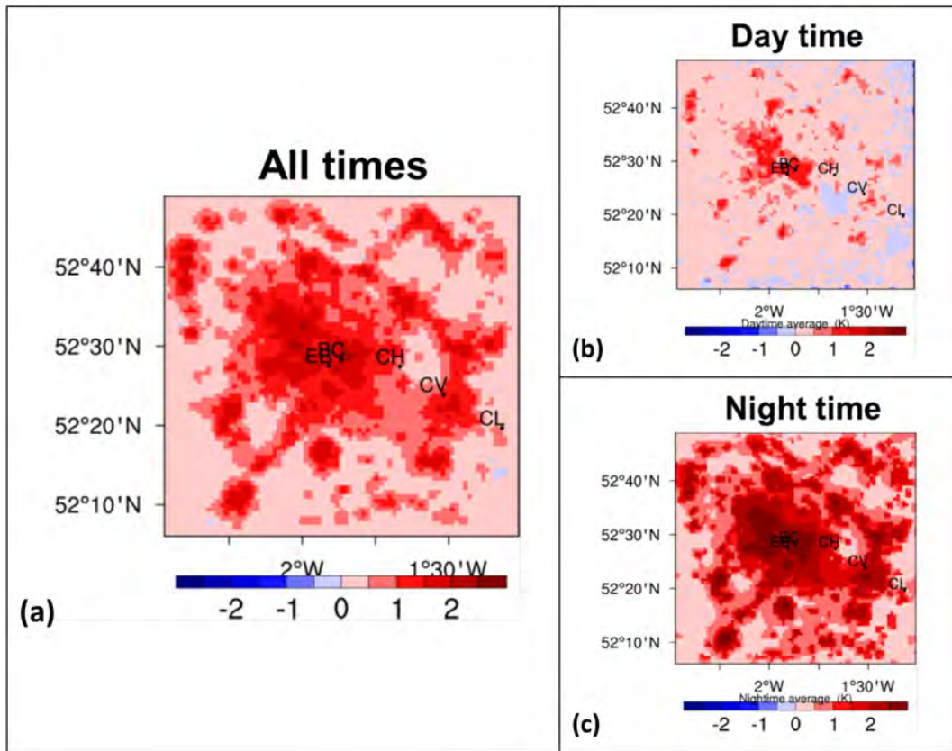
Fig. 5. (a) Average UHI intensity during heatwave periods (2–10 Aug 2003 and 16–27 July 2006) across the West Midlands; Averages over (b) daytime and (c) night time. Average UHI intensity was +2.1 °C (+1.4 °C in daytime, +2.9 °C at night time).
