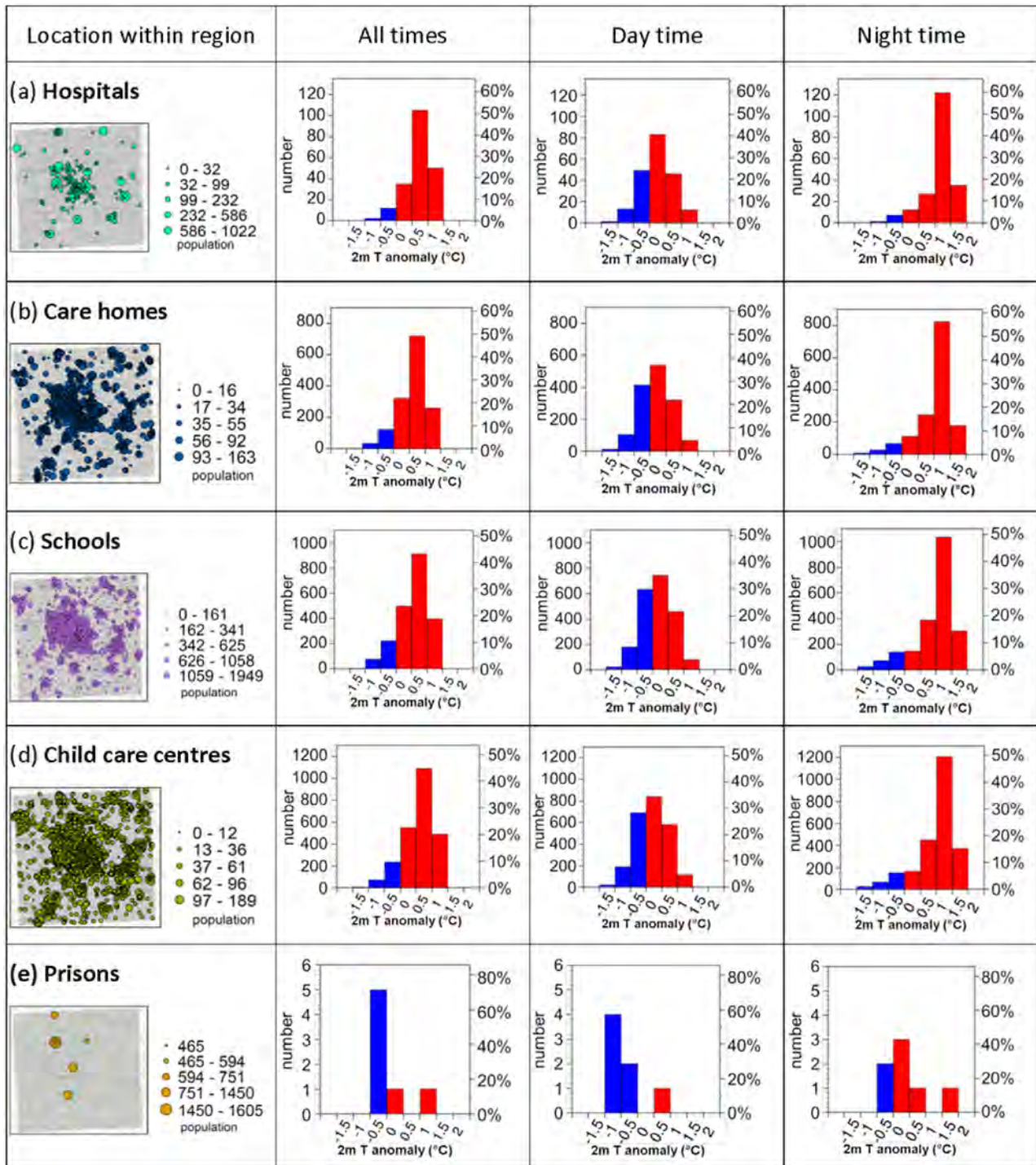
Fig. 9. Distribution of average ambient 2 m temperature at (a) hospitals, (b) care homes, (c) schools, (d) child care centres, and (e) prisons across the West Midlands. The first column shows the distribution of these locations across the West Midlands, and the next three columns represent the average anomaly averaged first across all times of day, and then broken down into average daytime anomaly (8 am–8 pm), and average night time anomaly (8 pm–8 am). The average temperature across the domain (used as the reference temperature) is 21.8 °C. Red = positive anomaly (warmer); Blue = negative (colder). (For interpretation of the references to colour in this figure legend, the reader is referred to the web version of this article.)
